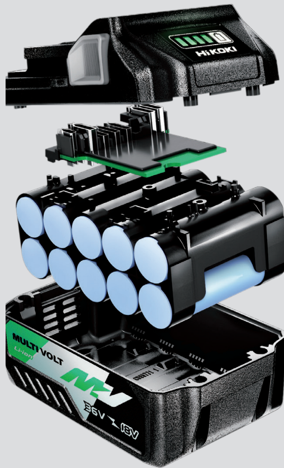
BSL36A18 / BSL36B18 MULTI VOLT Battery
